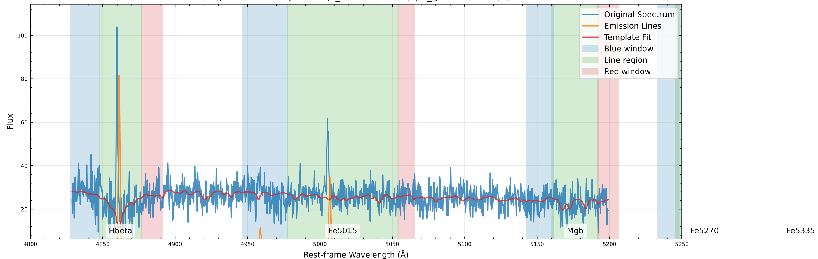
Original Data Comparison (v_star=-71.7 km/s, v_gas=-91.4 km/s)
