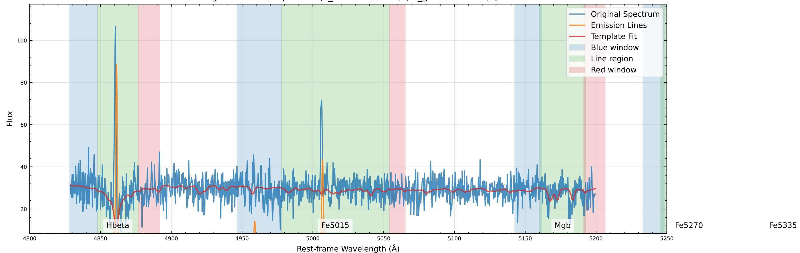
Original Data Comparison (v_star=-75.5 km/s, v_gas=-58.3 km/s)
