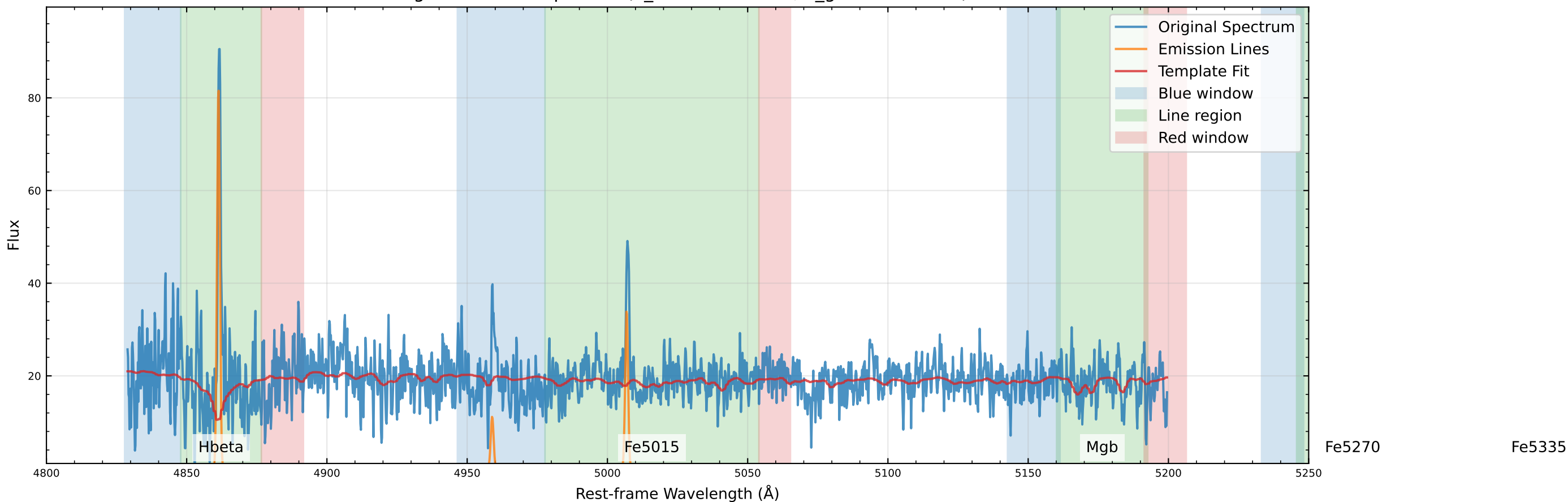
Original Data Comparison (v_star=33.5 km/s, v_gas=20.1 km/s)
