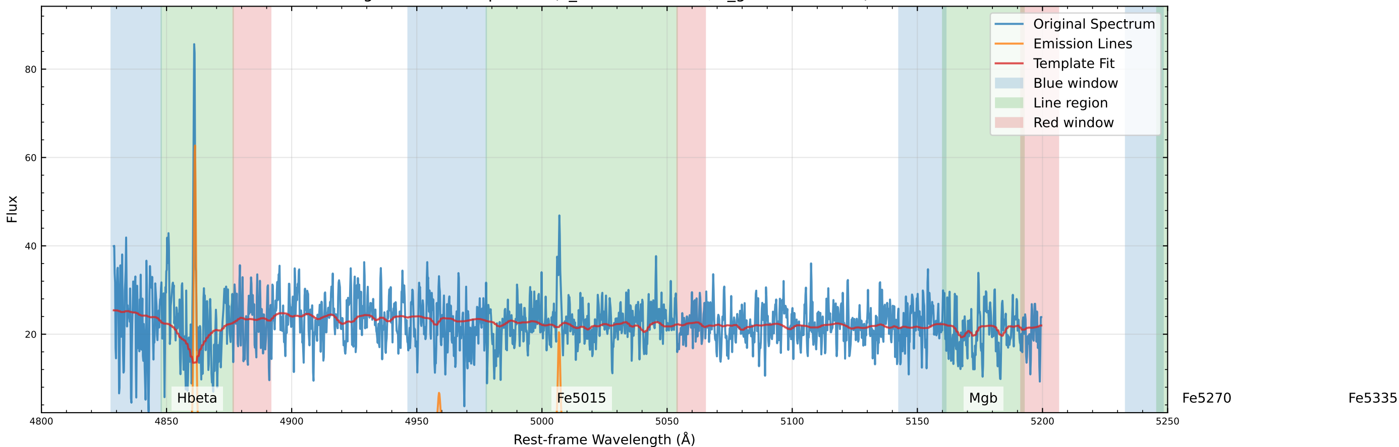
Original Data Comparison (v_star=-28.8 km/s, v_gas=-14.7 km/s)
