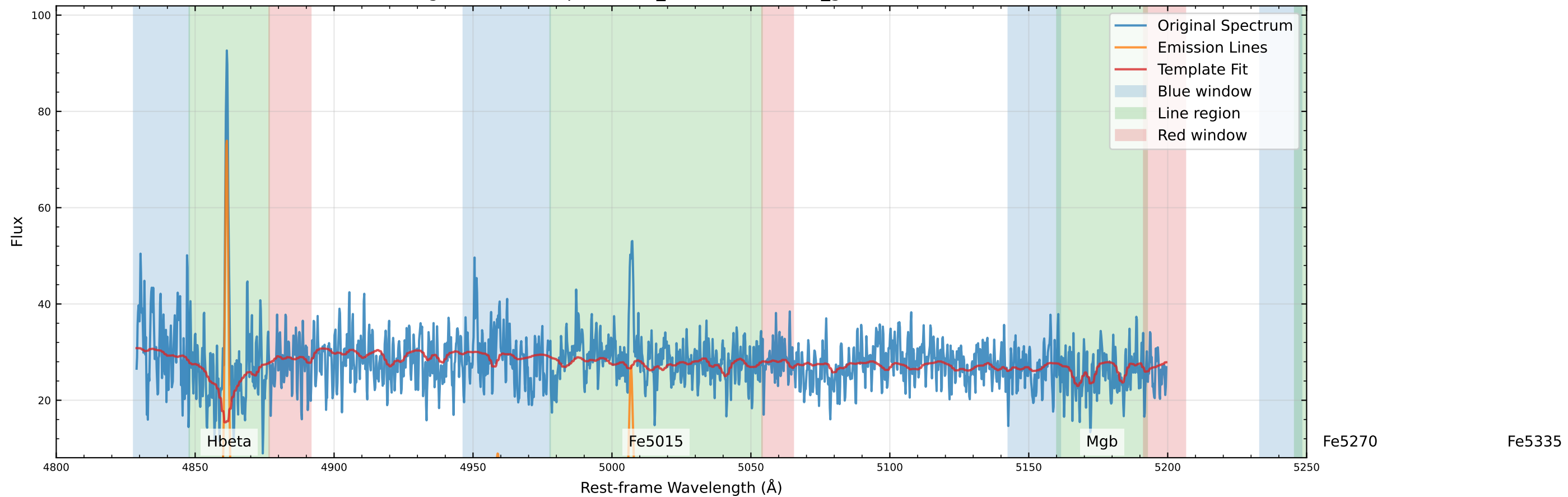
Original Data Comparison (v_star=-8.5 km/s, v_gas=4.0 km/s)
