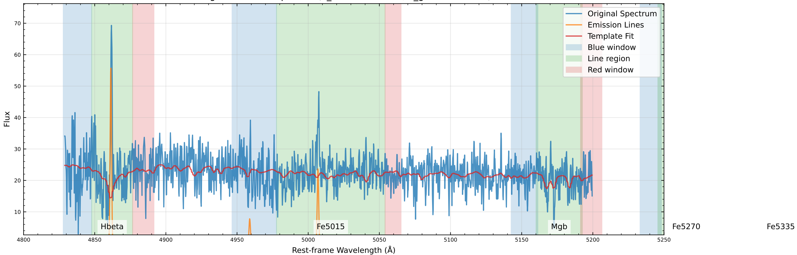
Original Data Comparison ( v_{\text{star}}=44.6 km/s, v_{\text{gas}}=24.8 km/s)
