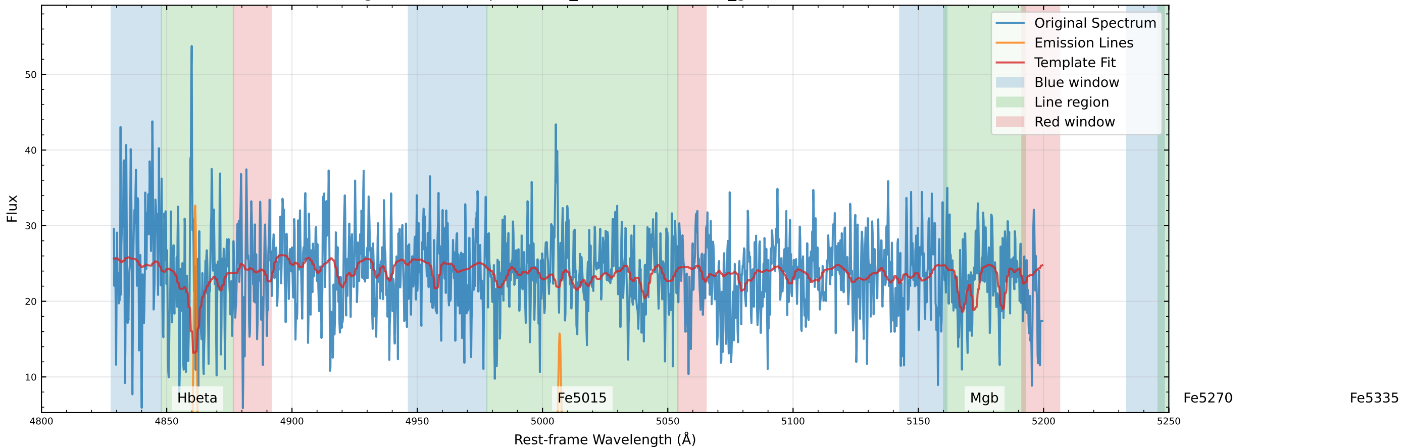
Original Data Comparison (v_star=-92.7 km/s, v_gas=-87.0 km/s)
