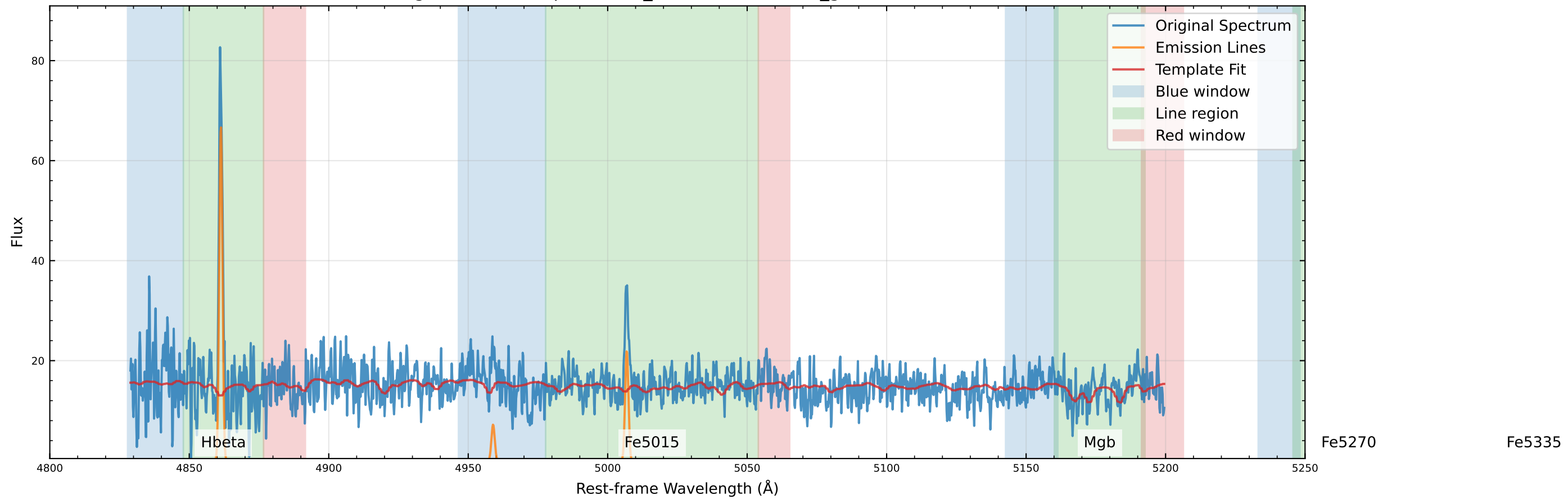
Original Data Comparison (v_star=-33.5 km/s, v_gas=-4.8 km/s)
