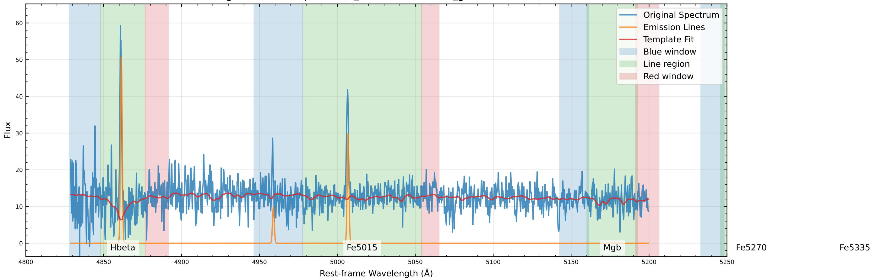
Original Data Comparison (v_star=-38.9 km/s, v_gas=-24.8 km/s)
