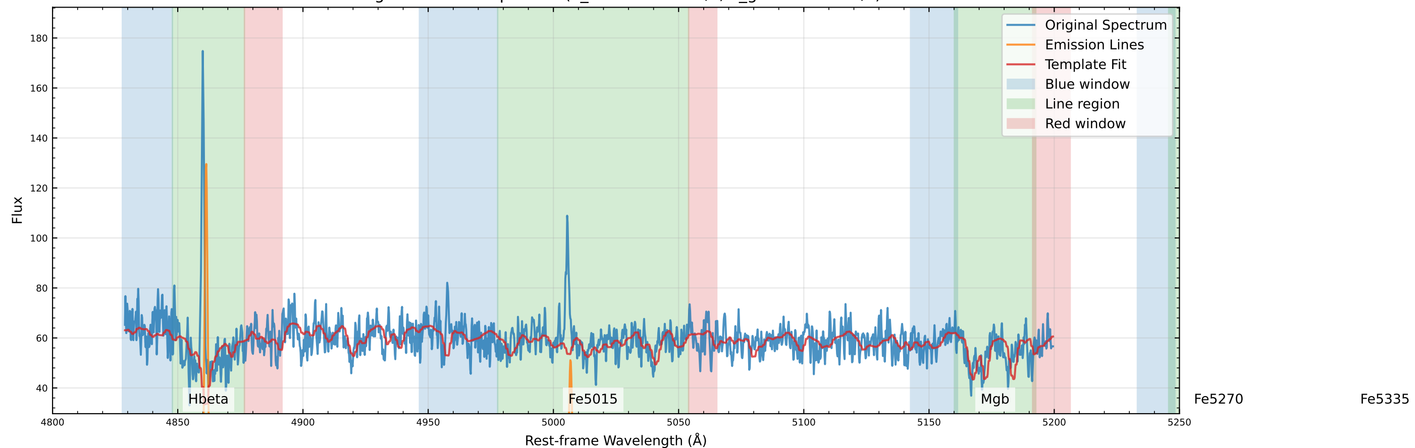
Original Data Comparison (v_star=-80.0 km/s, v_gas=-81.8 km/s)
