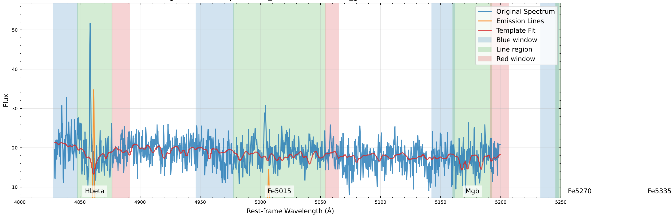
Original Data Comparison (v_star=-169.9 km/s, v_gas=-175.4 km/s)
