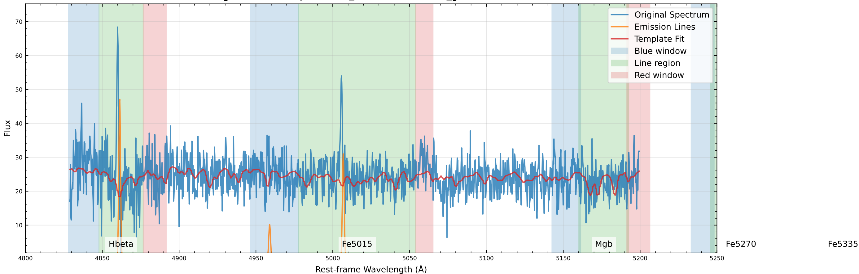
Original Data Comparison (v_star=-91.7 km/s, v_gas=-81.3 km/s)
