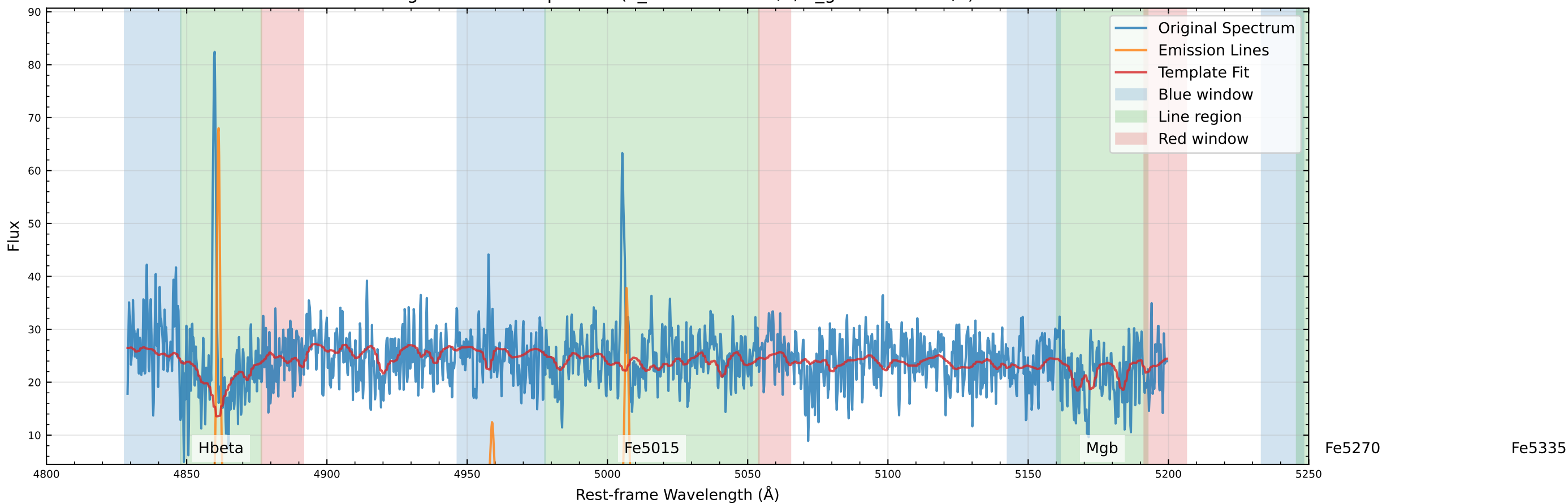
Original Data Comparison (v_star=-75.5 km/s, v_gas=-86.6 km/s)
