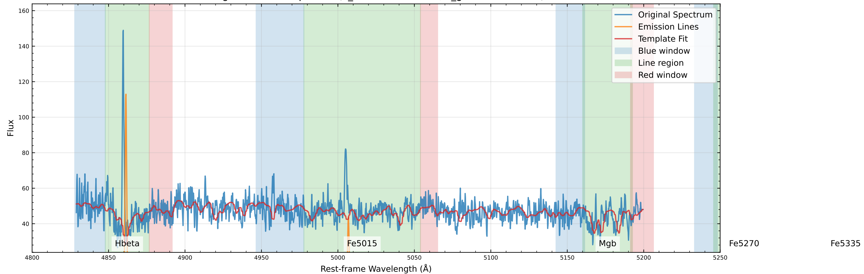
Original Data Comparison (v_star=-121.1 km/s, v_gas=-108.6 km/s)
