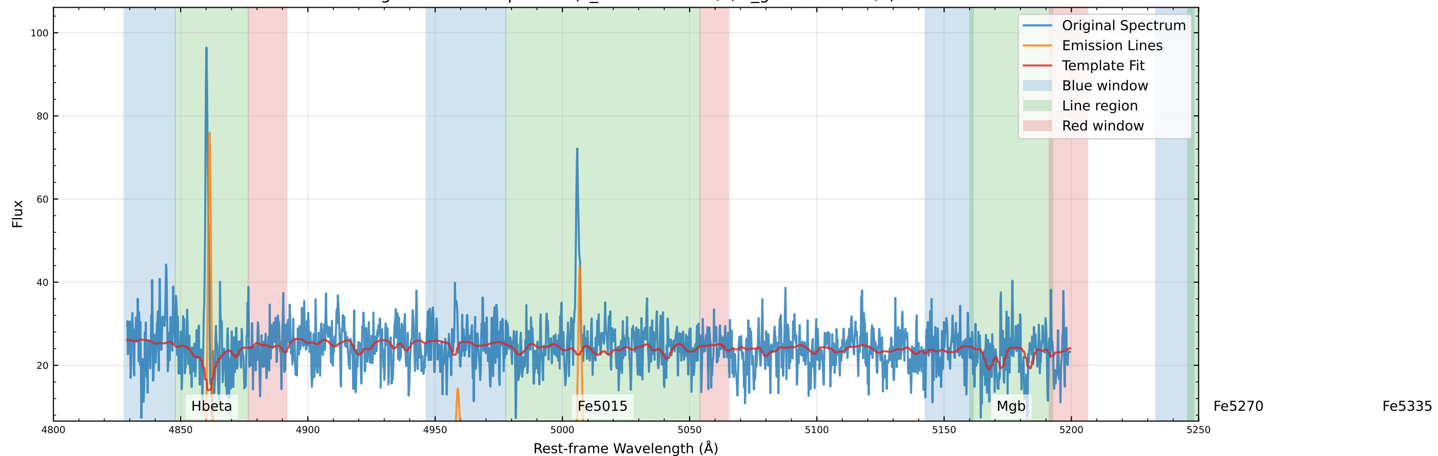
Original Data Comparison (v_star=-85.9 km/s, v_gas=-65.0 km/s)
