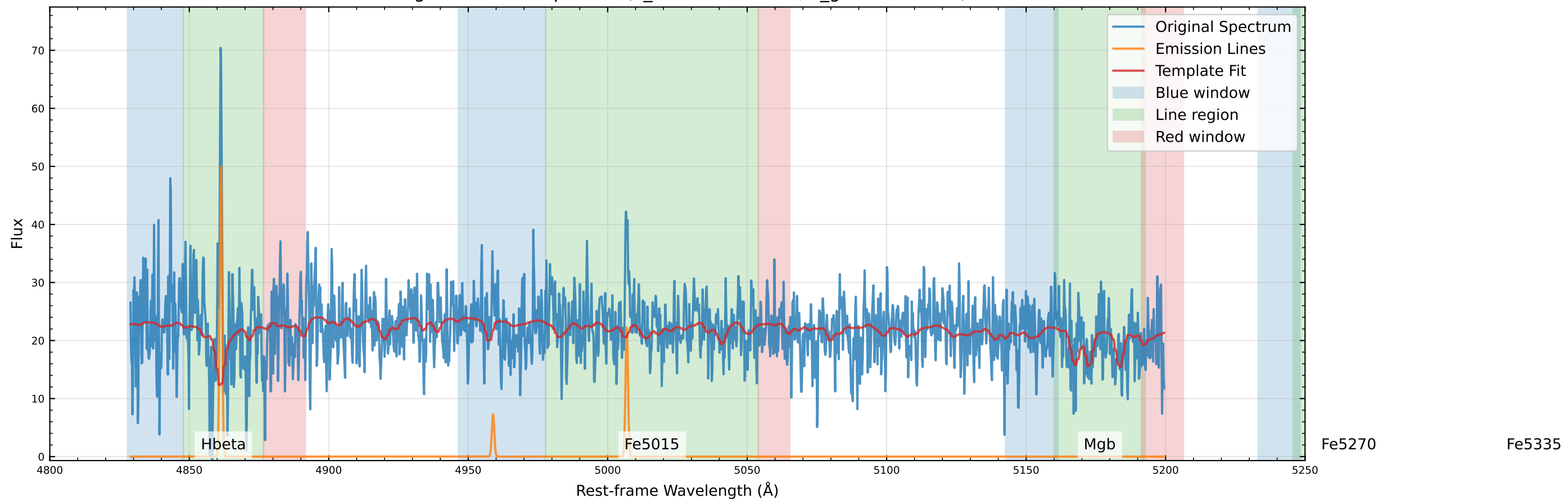
Original Data Comparison (v_star=-18.7 km/s, v_gas=-4.3 km/s)
