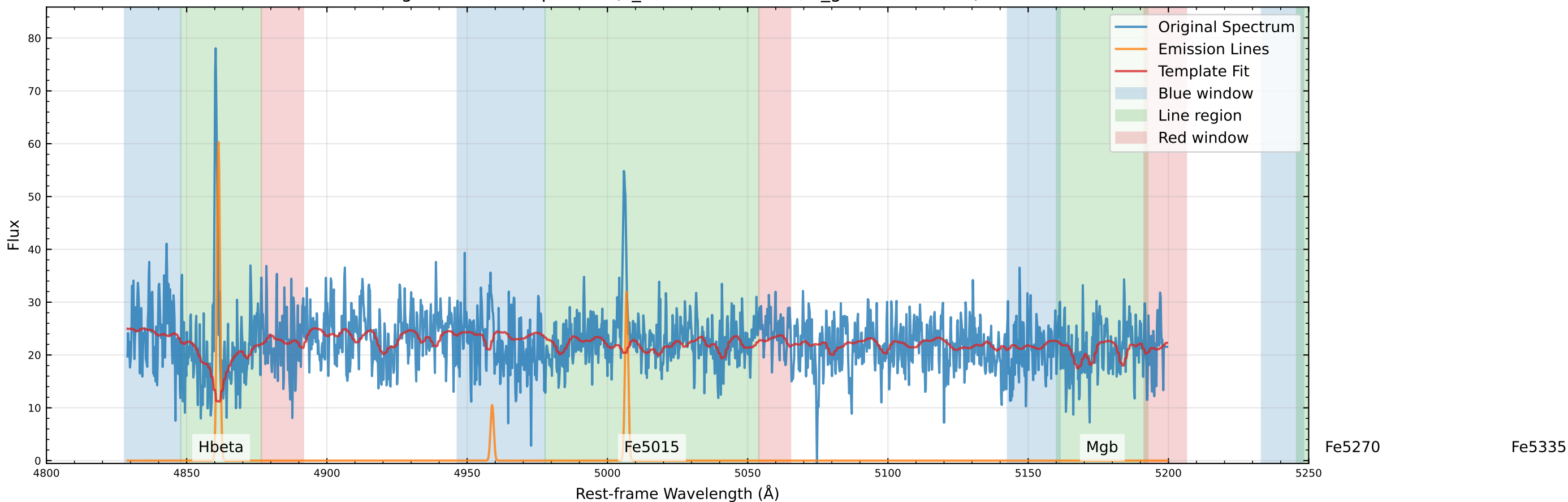
Original Data Comparison (v_star=-118.1 km/s, v_gas=-54.6 km/s)
