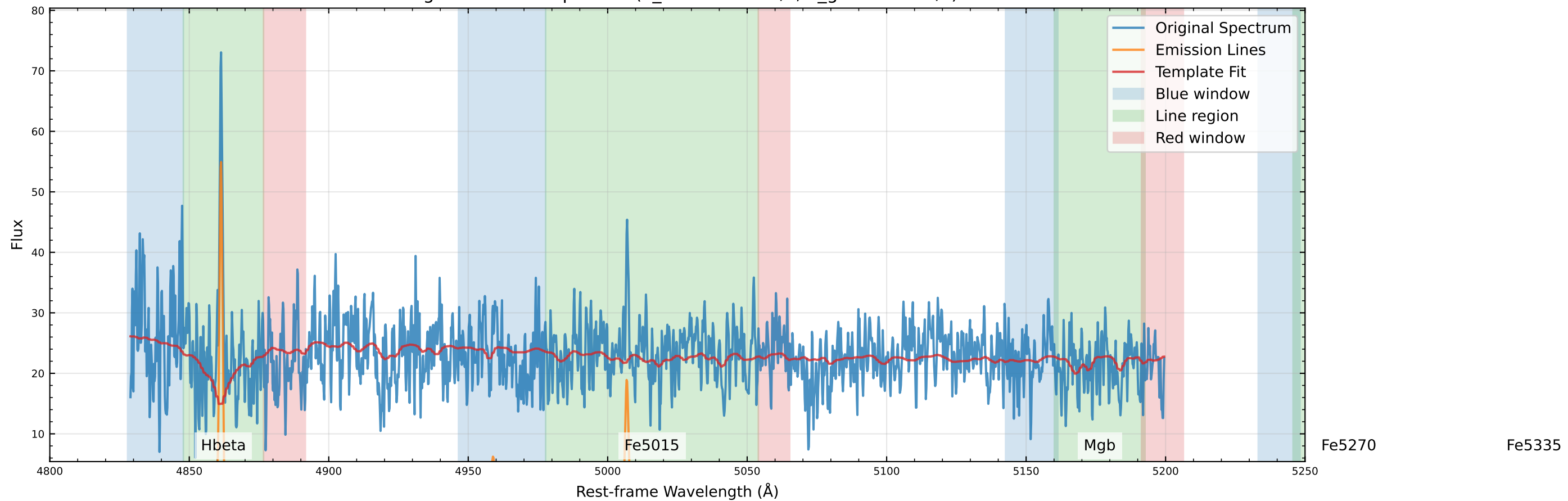
Original Data Comparison (v_star=-8.3 km/s, v_gas=3.4 km/s)
