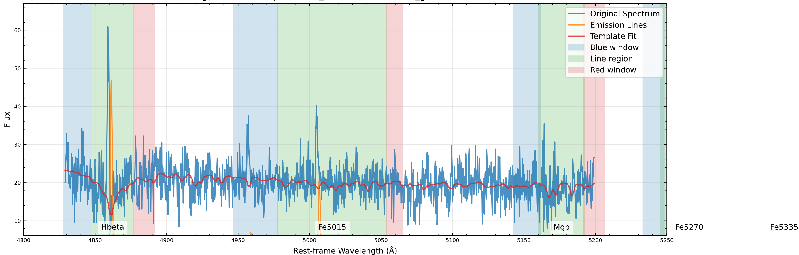
Original Data Comparison (v_star=-123.4 km/s, v_gas=-132.7 km/s)
