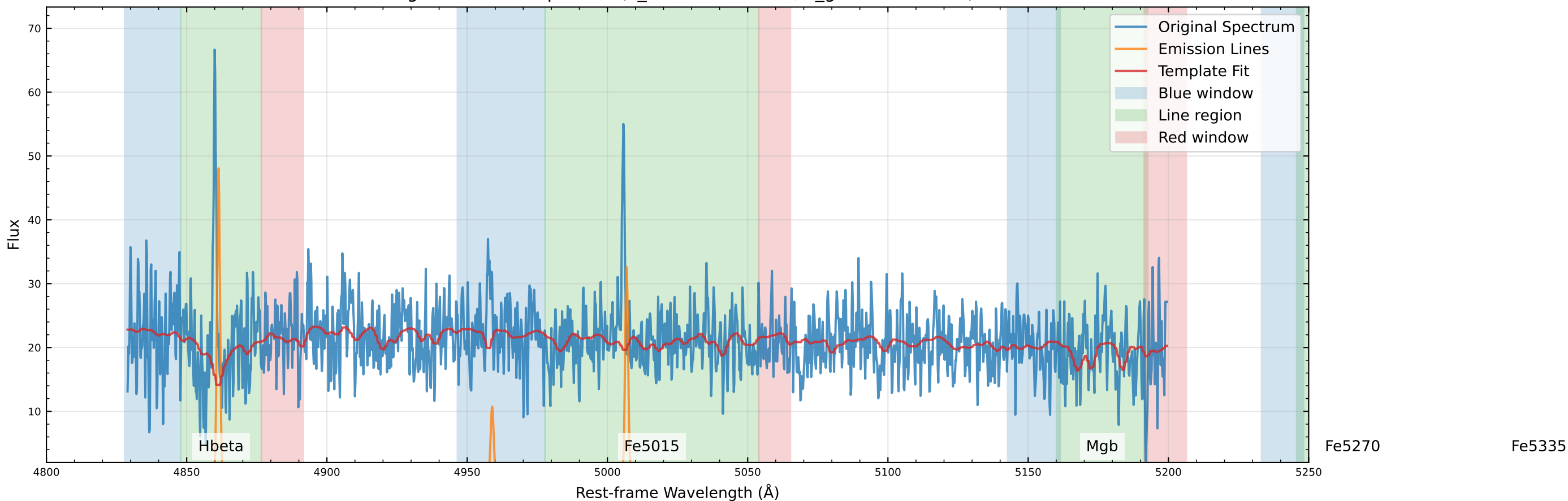
Original Data Comparison (v_star=-64.8 km/s, v_gas=-76.5 km/s)
