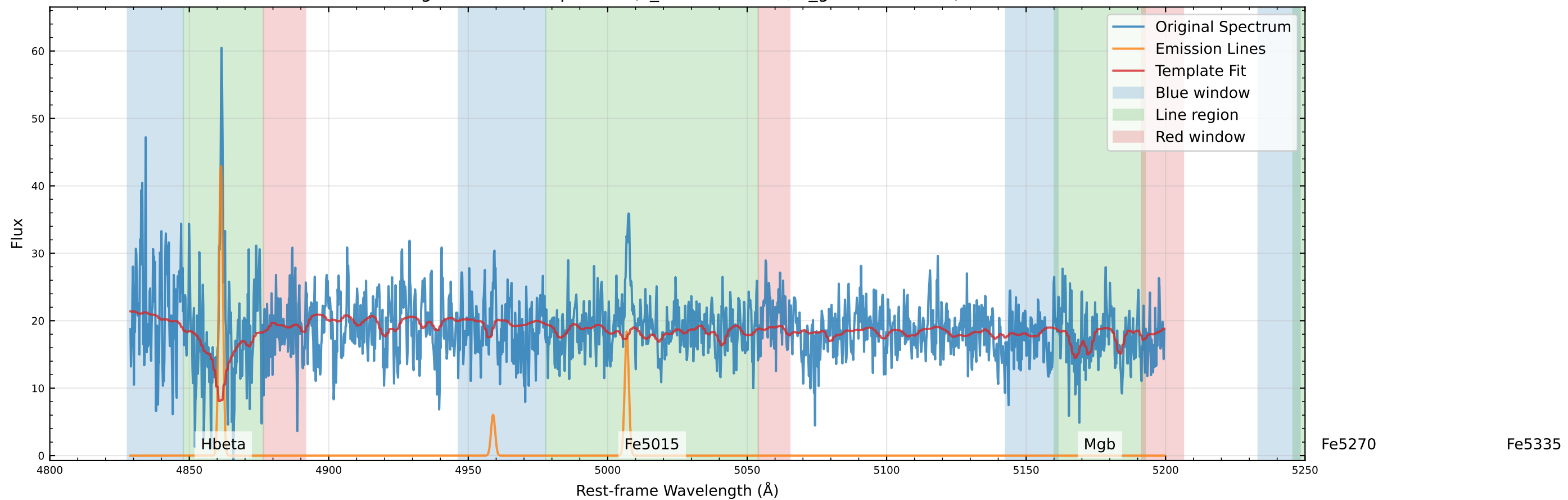
Original Data Comparison (v_star=7.7 km/s, v_gas=18.5 km/s)
