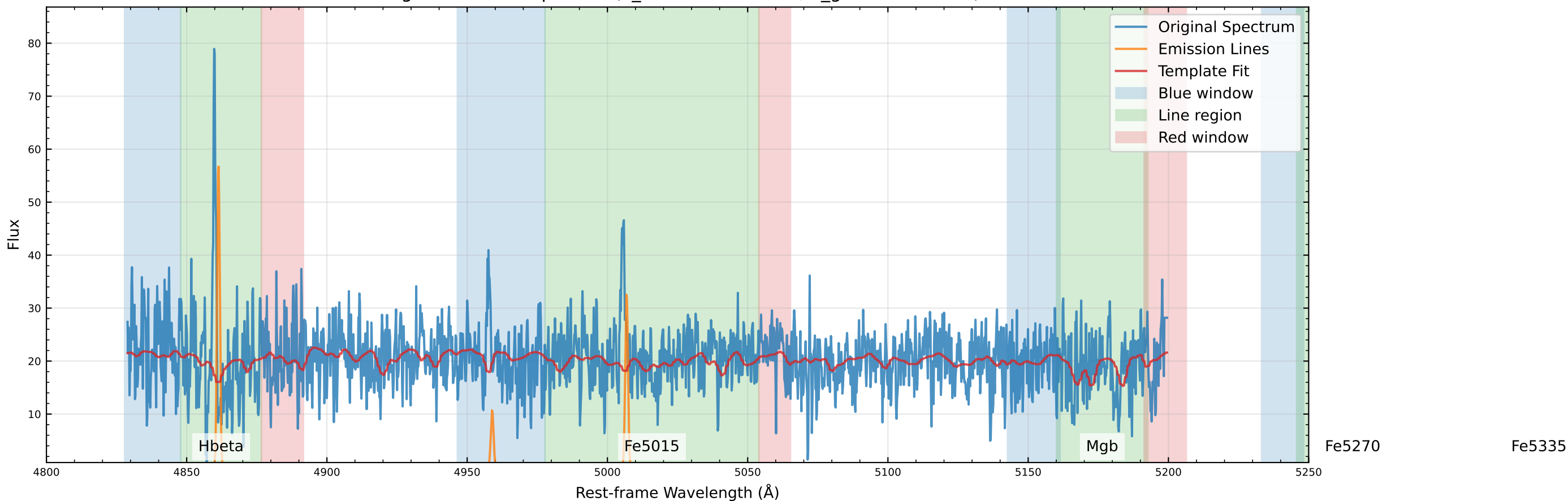
Original Data Comparison (v_star=-108.0 km/s, v_gas=-87.8 km/s)
