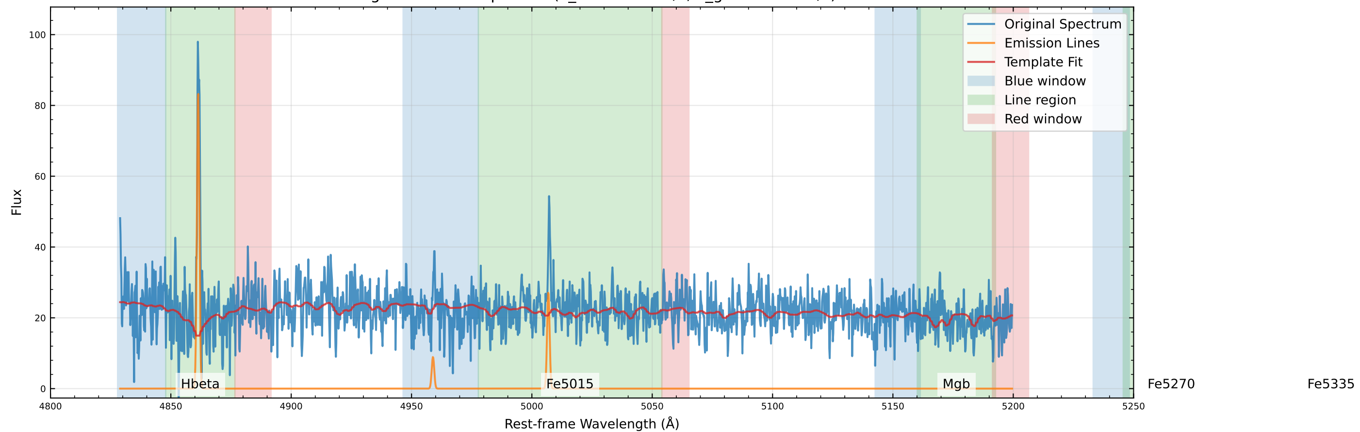
Original Data Comparison (v_star=0.4 km/s, v_gas=11.2 km/s)
