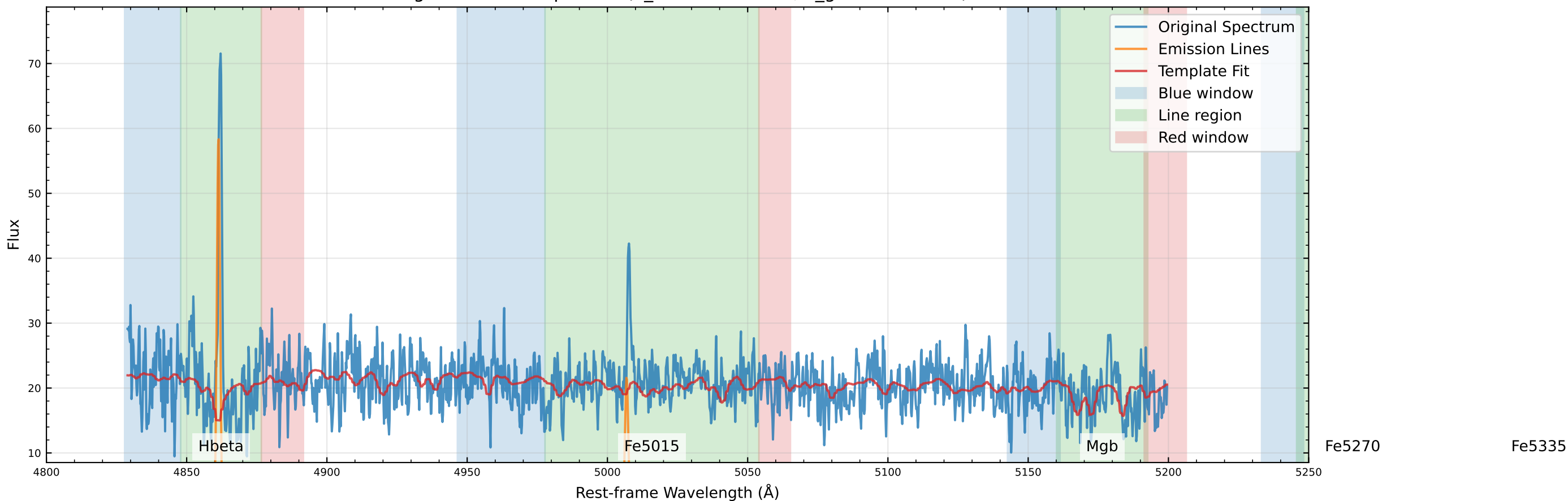
Original Data Comparison (v_star=66.7 km/s, v_gas=39.3 km/s)
