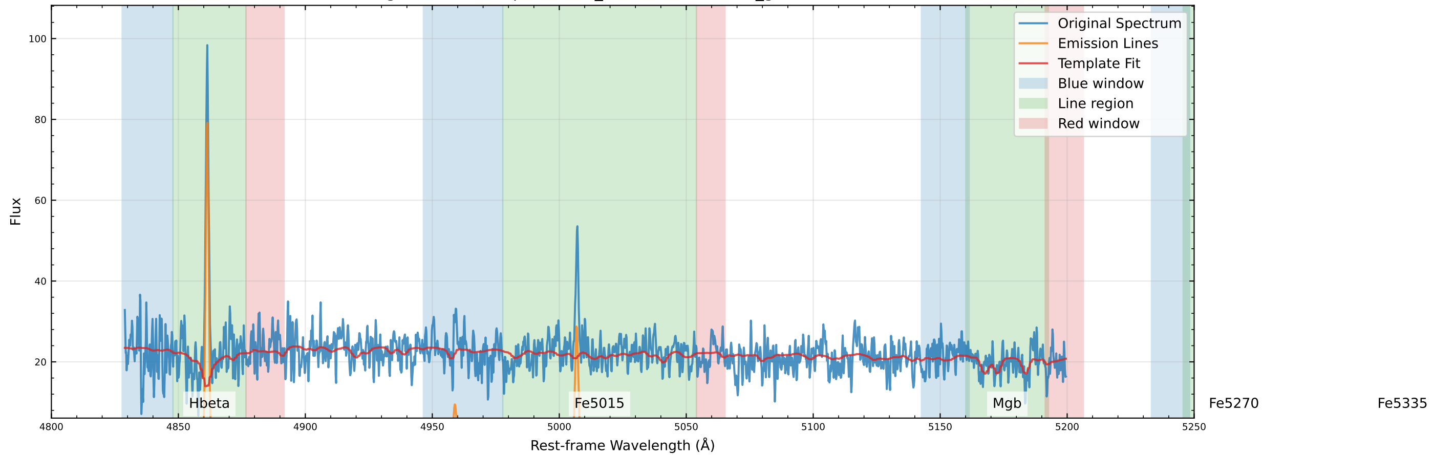
Original Data Comparison (v_star=-19.2 km/s, v_gas=1.5 km/s)
