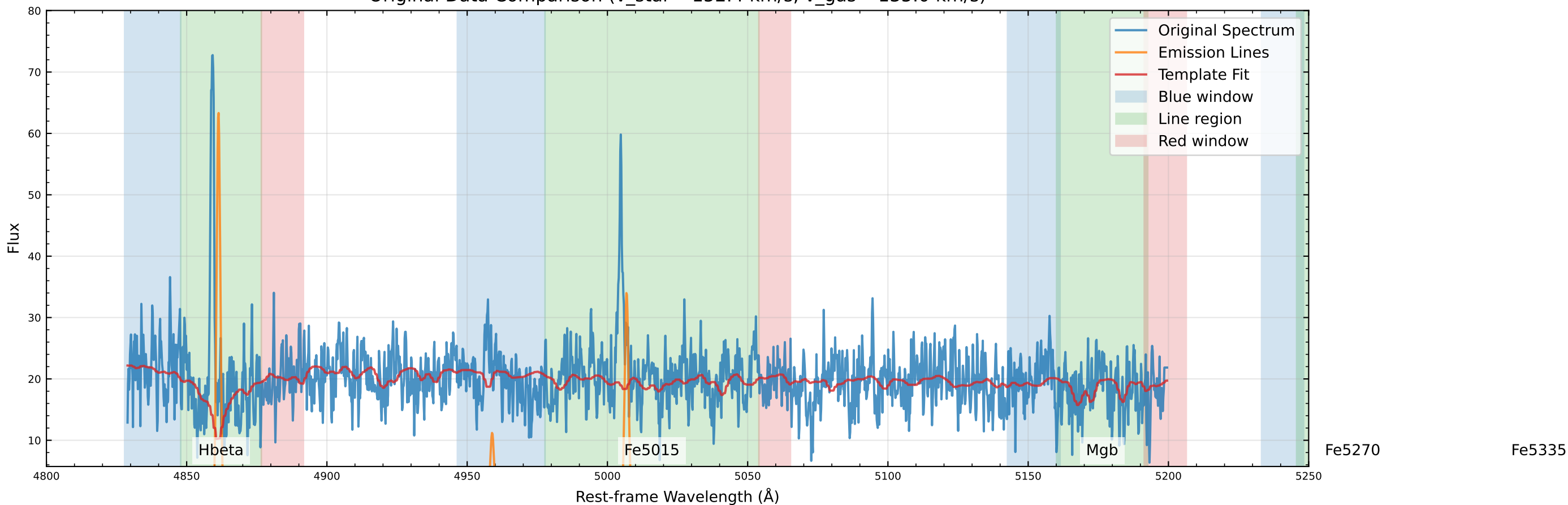
Original Data Comparison (v_star=-152.4 km/s, v_gas=-135.0 km/s)
