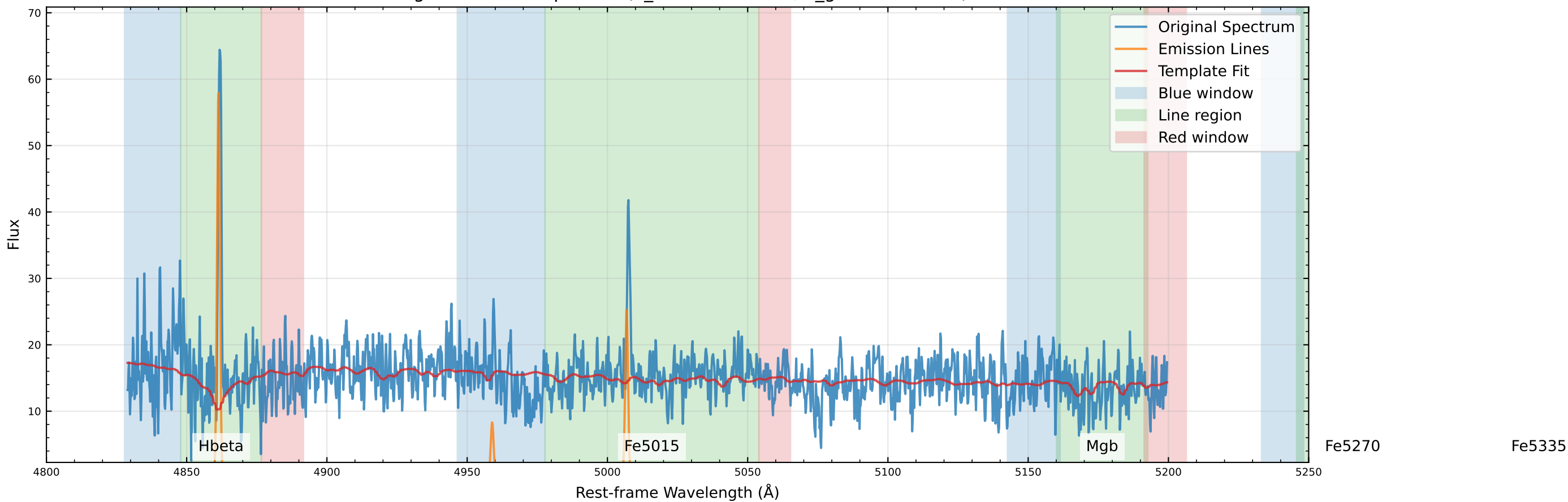
Original Data Comparison (v_star=50.6 km/s, v_gas=32.3 km/s)
