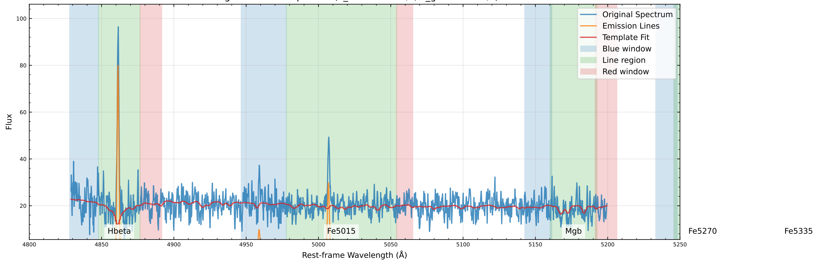
Original Data Comparison (v_star=0.1 km/s, v_gas=6.9 km/s)
