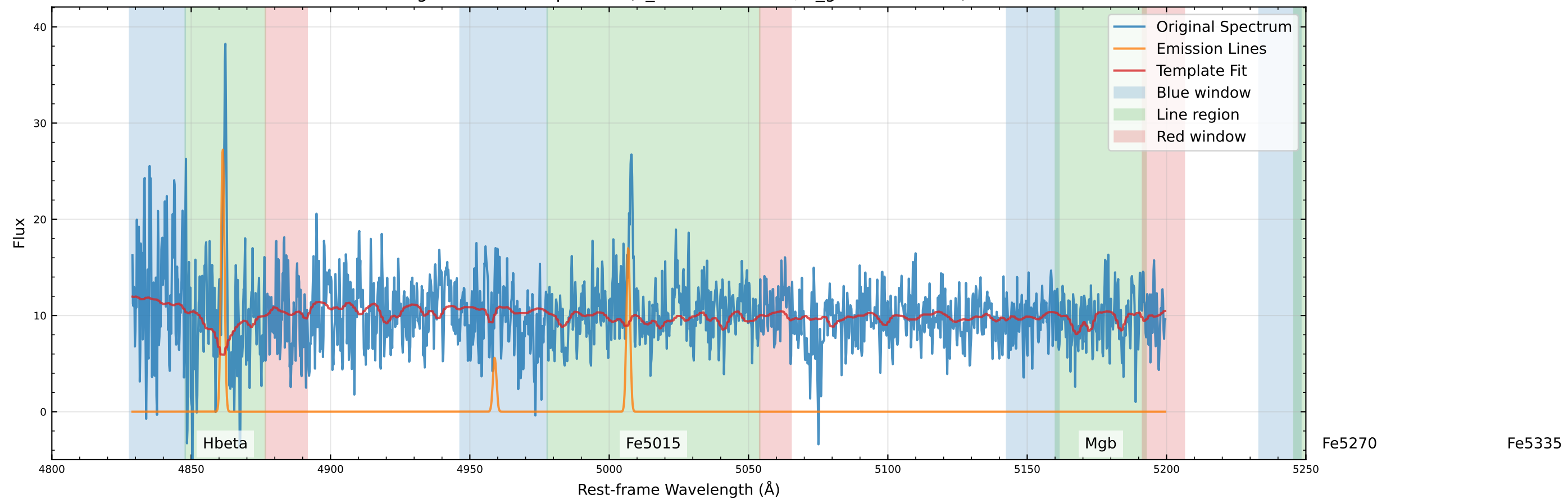
Original Data Comparison (v_star=59.4 km/s, v_gas=48.3 km/s)
