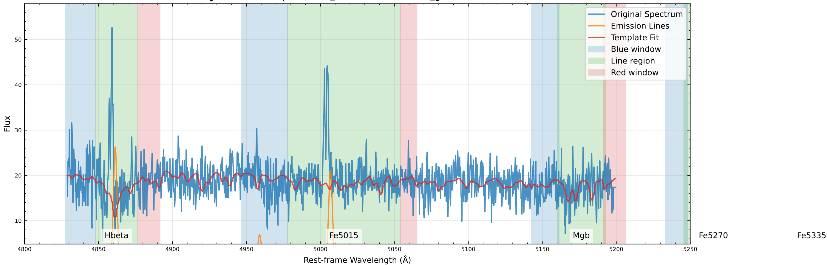
Original Data Comparison (v_star=-217.9 km/s, v_gas=-158.7 km/s)
