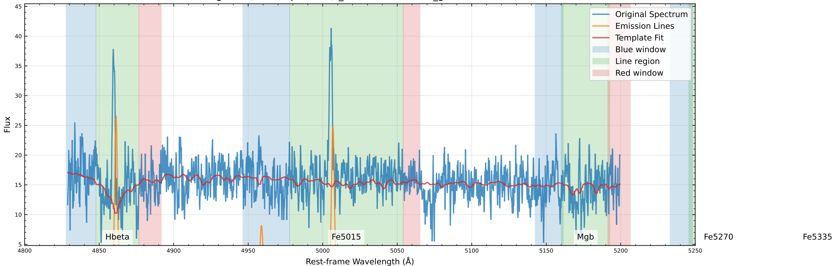
Original Data Comparison (v_star=-89.6 km/s, v_gas=-93.2 km/s)
