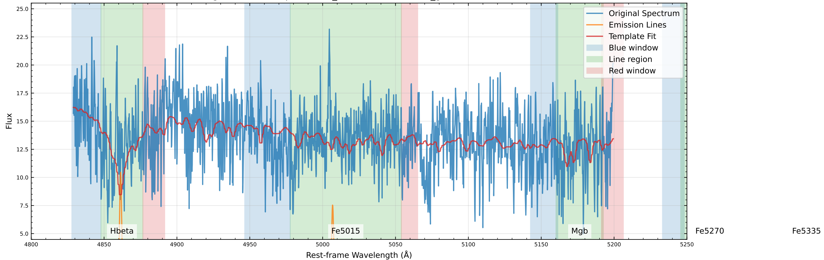
Original Data Comparison (v_star=-170.7 km/s, v_gas=-156.9 km/s)
