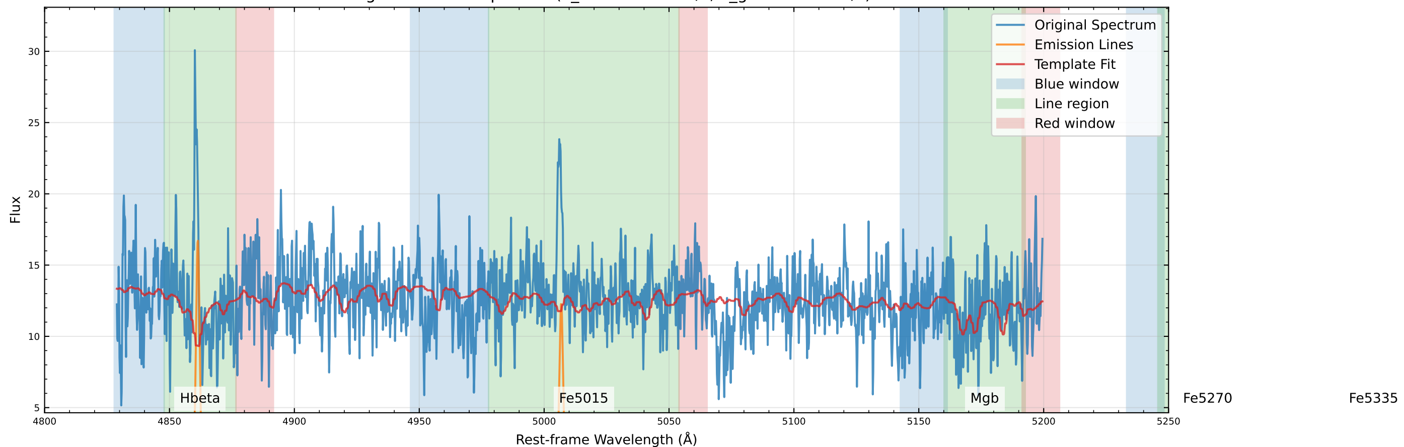
Original Data Comparison (v_star=-59.3 km/s, v_gas=-46.8 km/s)
