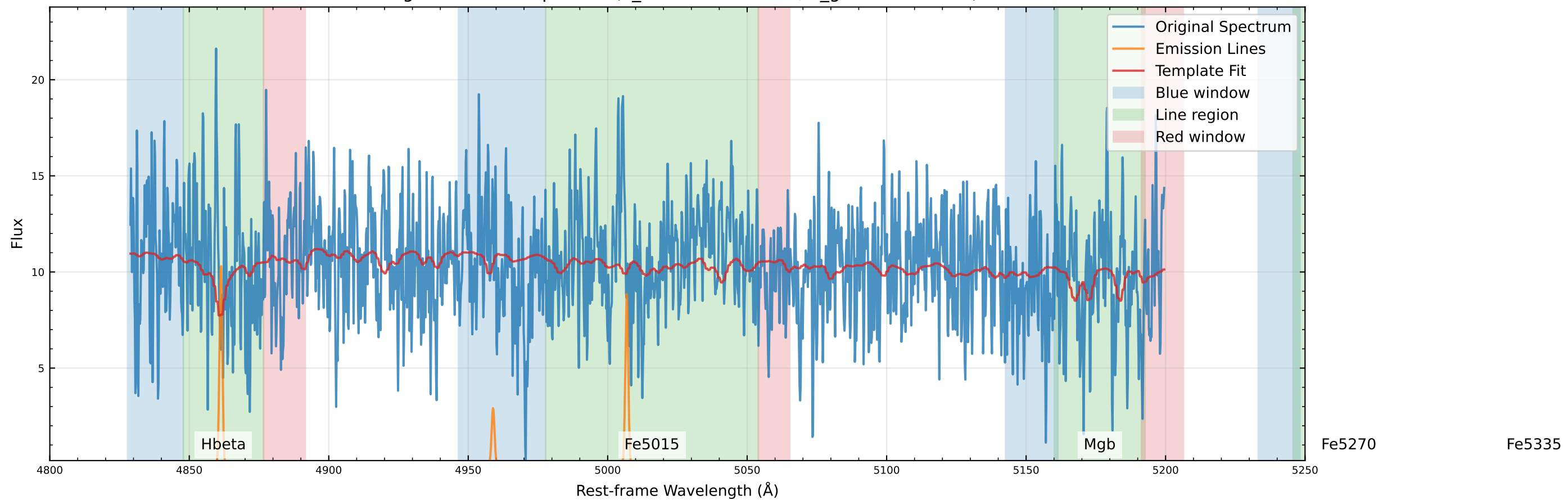
Original Data Comparison (v_star=-122.2 km/s, v_gas=-98.6 km/s)
