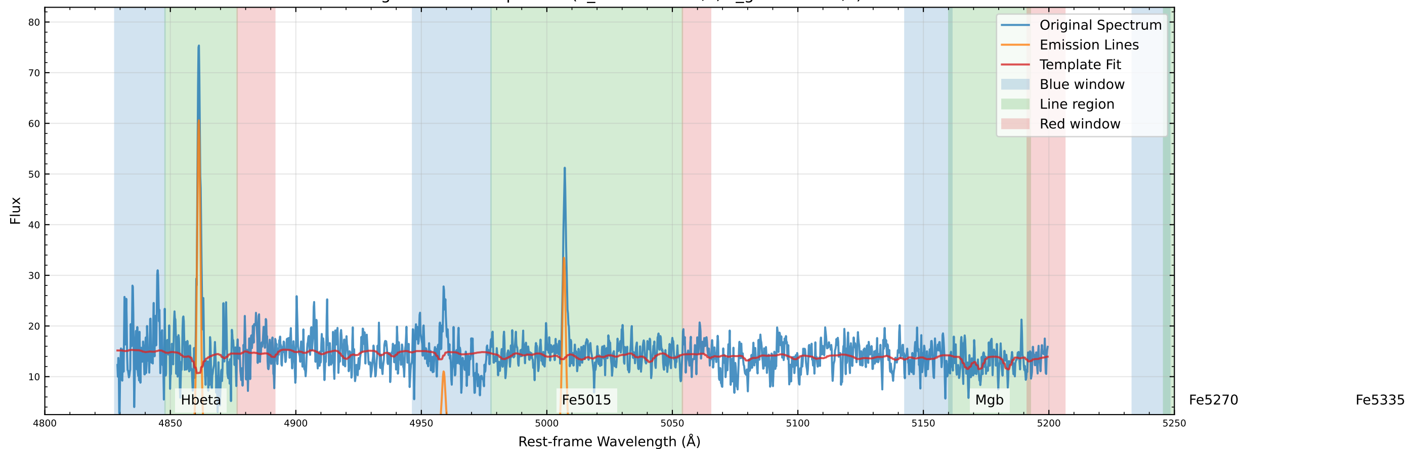
Original Data Comparison (v_star=-2.6 km/s, v_gas=8.2 km/s)
