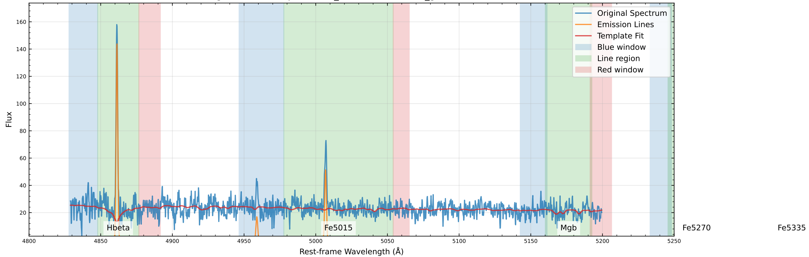
Original Data Comparison (v_star=-27.1 km/s, v_gas=-2.3 km/s)
