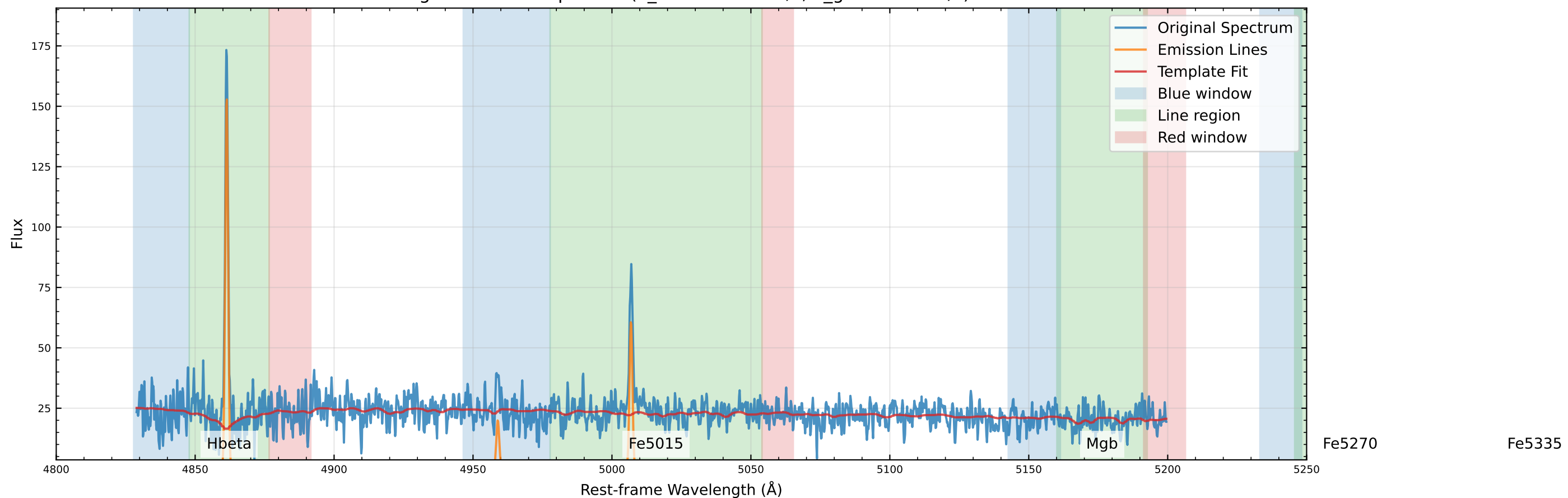
Original Data Comparison (v_star=-28.7 km/s, v_gas=-1.2 km/s)
