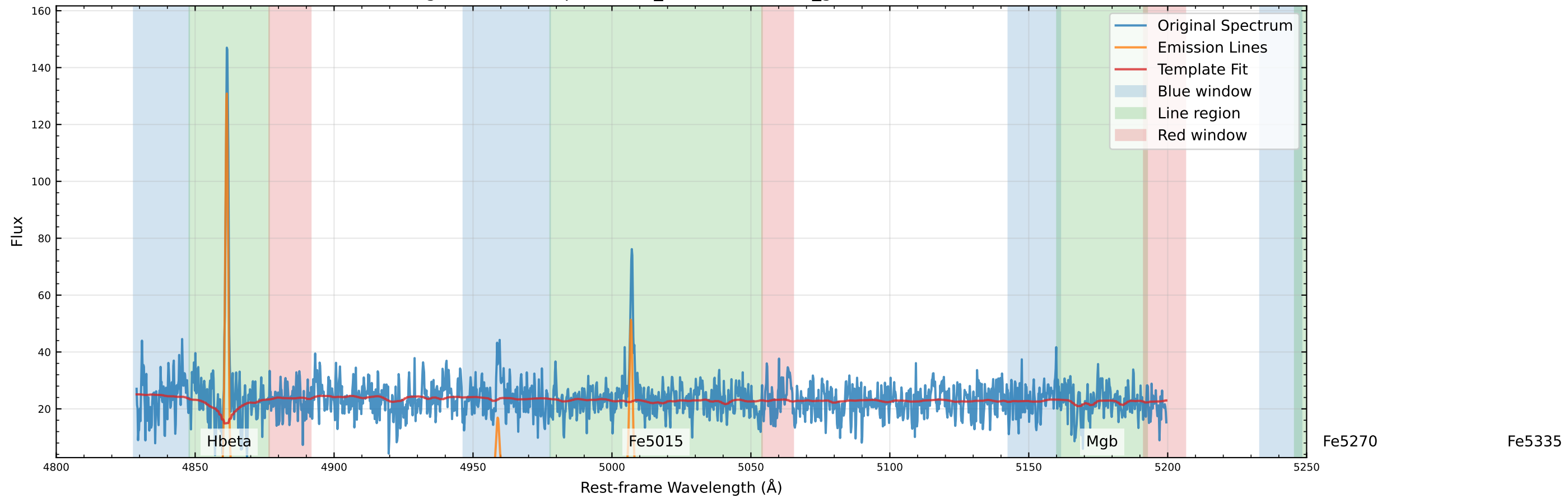
Original Data Comparison (v_star=3.7 km/s, v_gas=10.2 km/s)
