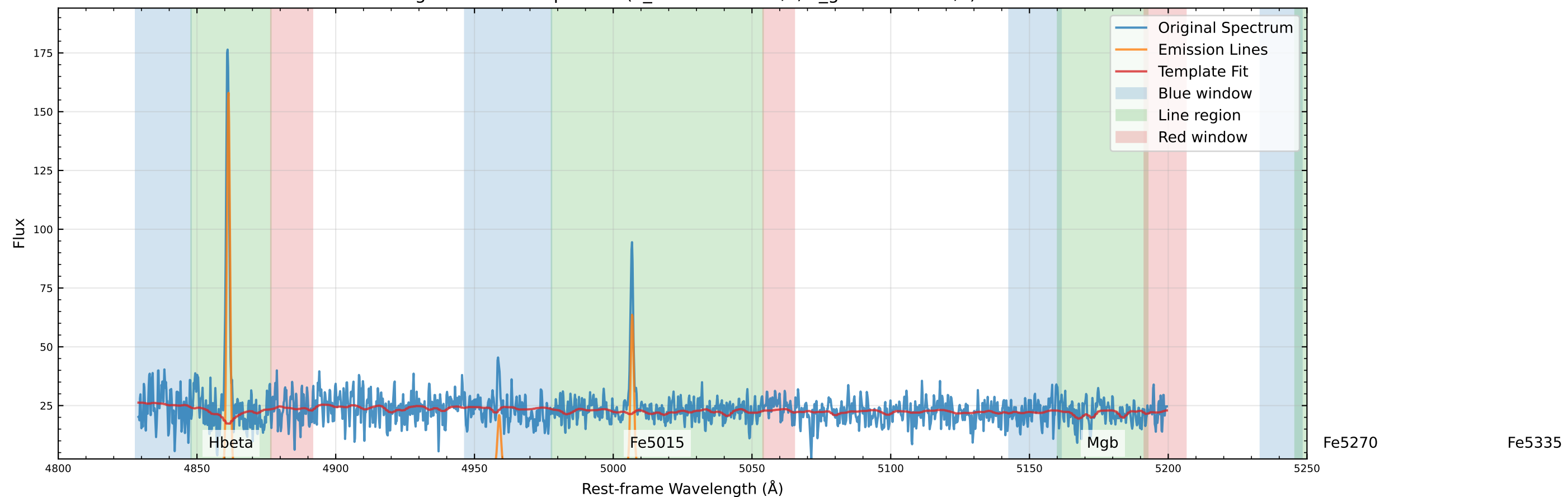
Original Data Comparison (v_star=-56.6 km/s, v_gas=-16.6 km/s)
