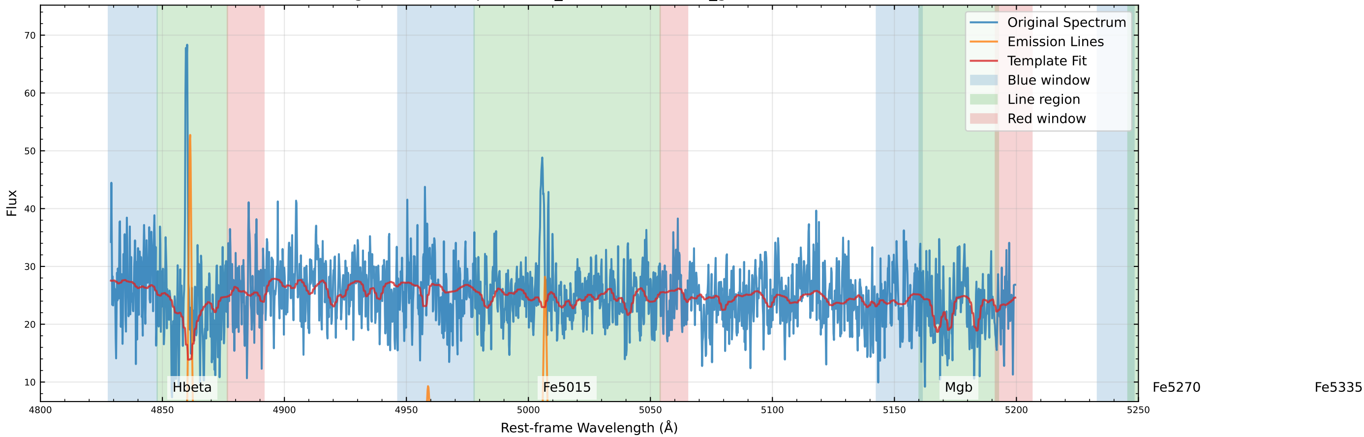
Original Data Comparison (v_star=-63.1 km/s, v_gas=-86.8 km/s)
