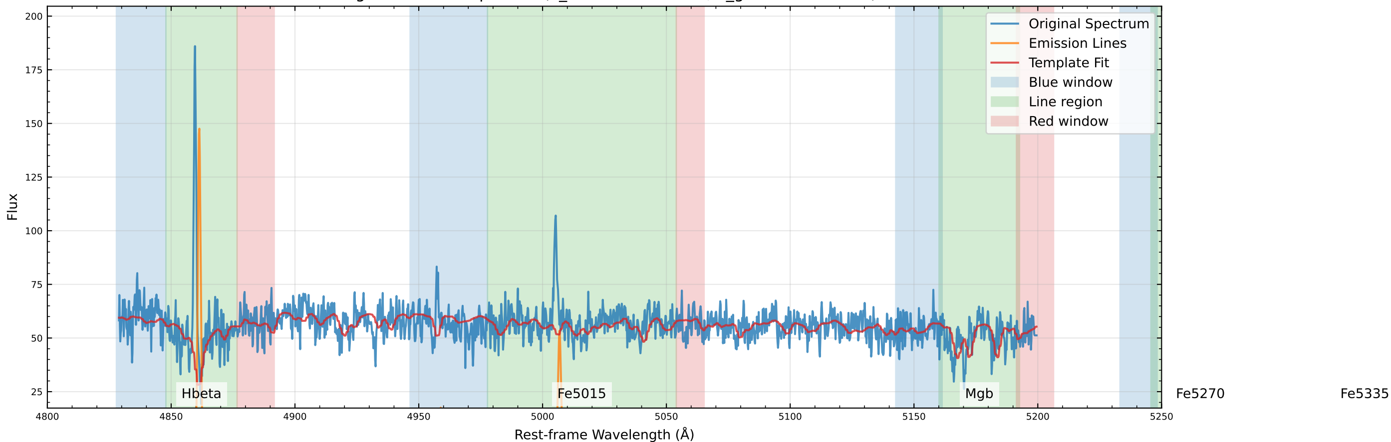
Original Data Comparison (v_star=-106.5 km/s, v_gas=-104.4 km/s)
