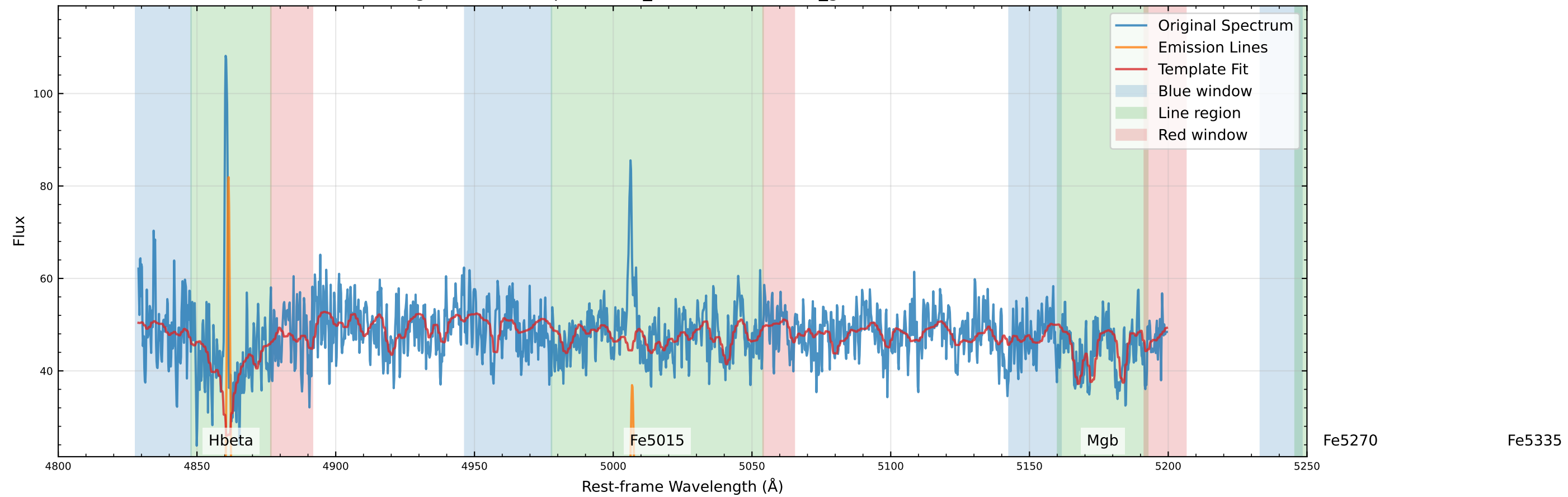
Original Data Comparison (v_star=-58.0 km/s, v_gas=-50.3 km/s)
