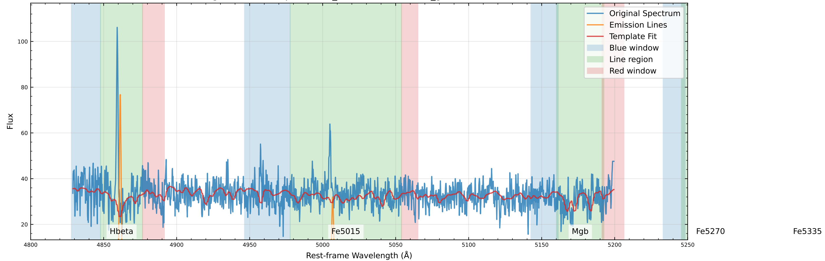
Original Data Comparison (v_star=-112.0 km/s, v_gas=-123.1 km/s)
