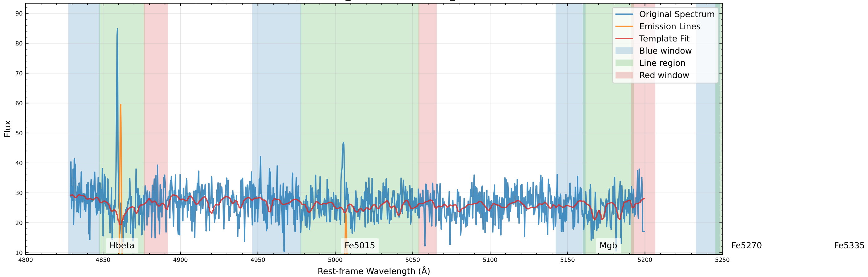
Original Data Comparison (v_star=-160.3 km/s, v_gas=-134.6 km/s)
