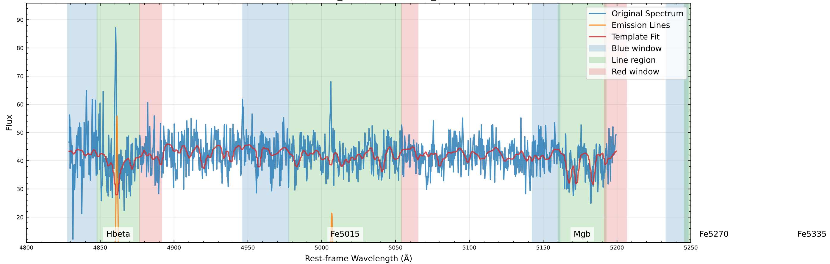
Original Data Comparison (v_star=-71.1 km/s, v_gas=-55.8 km/s)
