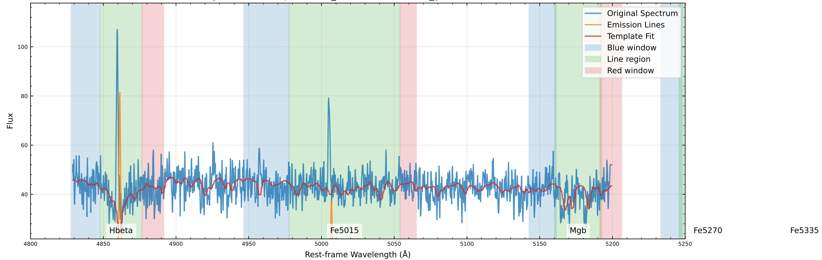
Original Data Comparison (v_star=-120.9 km/s, v_gas=-106.0 km/s)
