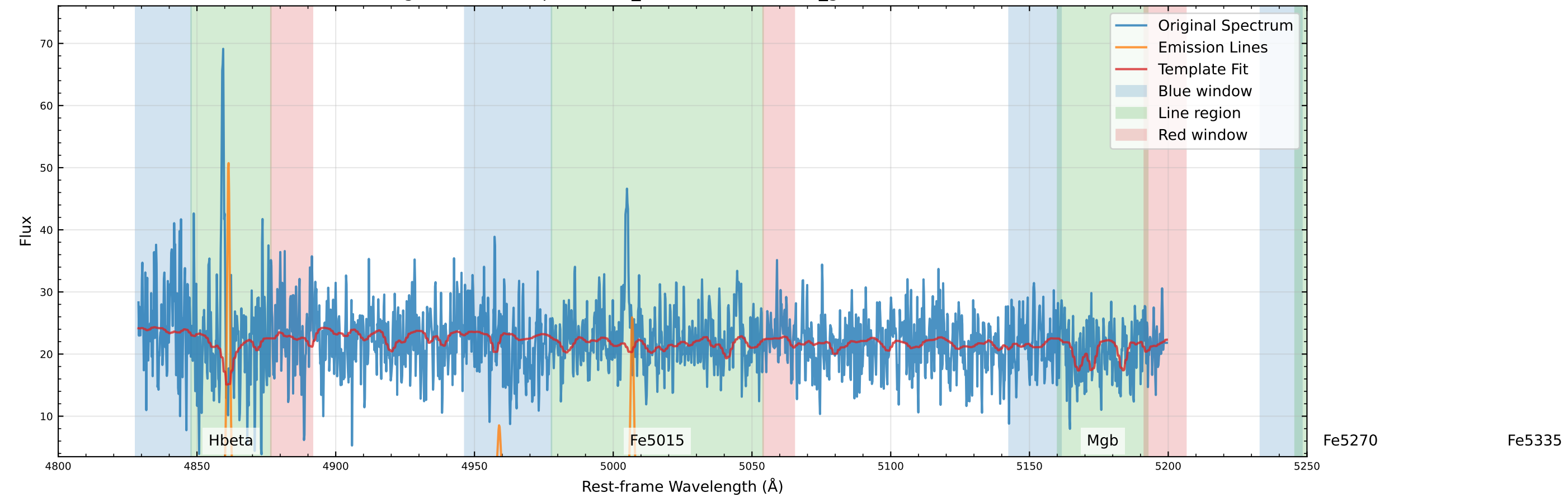
Original Data Comparison (v_star=-113.4 km/s, v_gas=-123.3 km/s)
