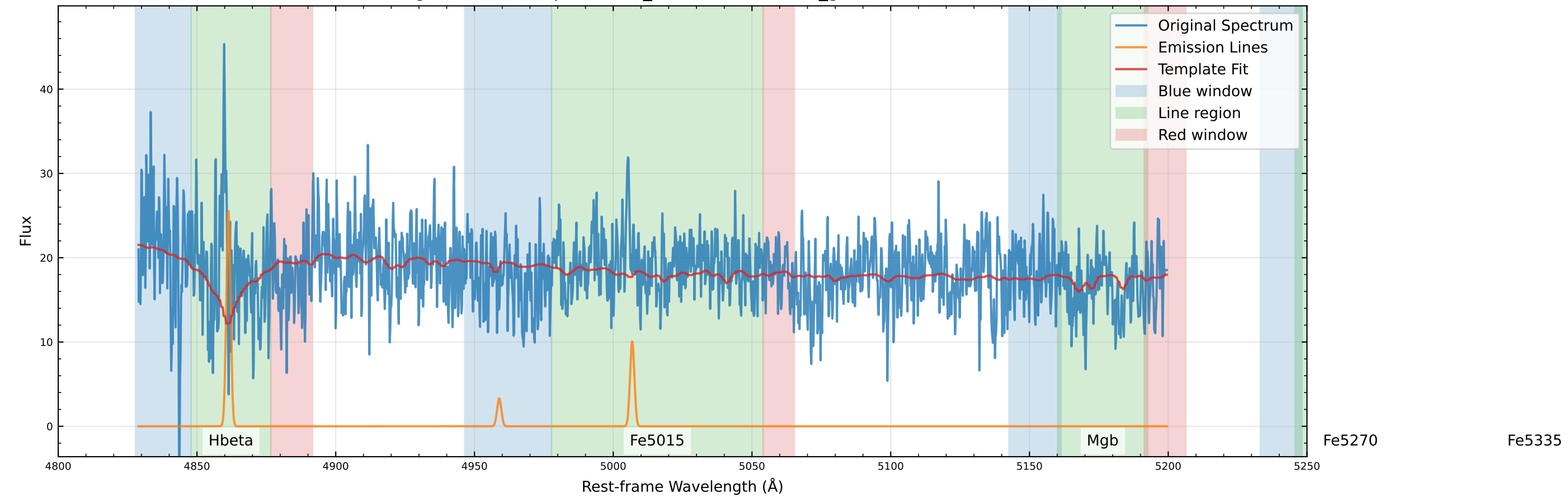
Original Data Comparison (v_star=-93.5 km/s, v_gas=-99.7 km/s)
