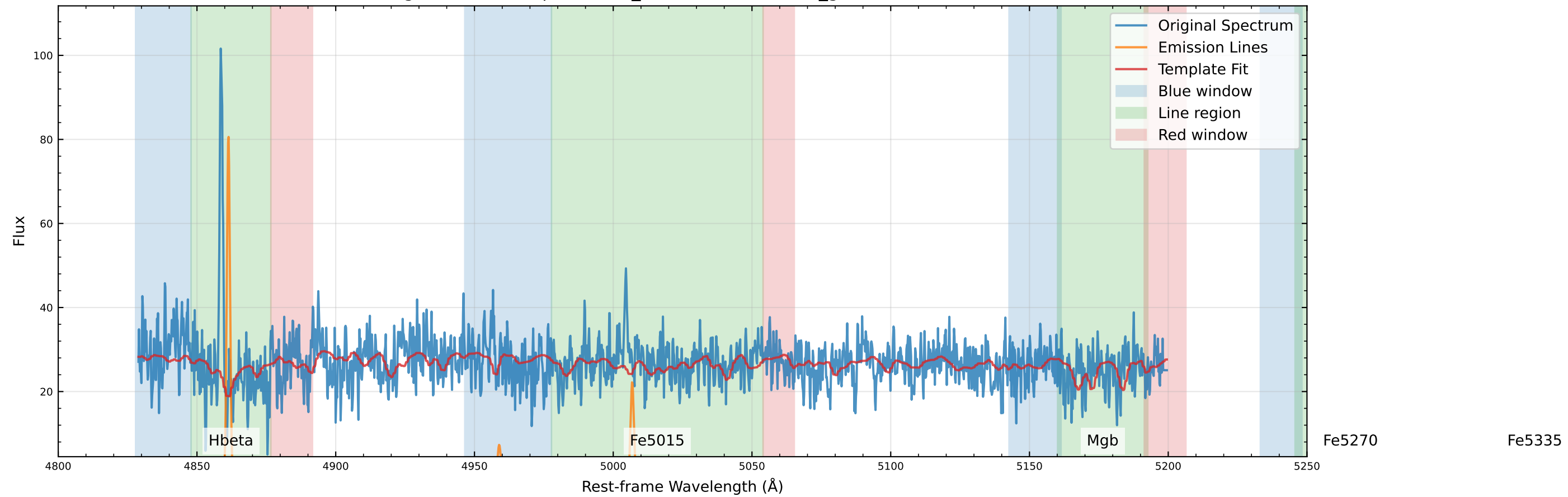
Original Data Comparison (v_star=-146.6 km/s, v_gas=-158.8 km/s)
