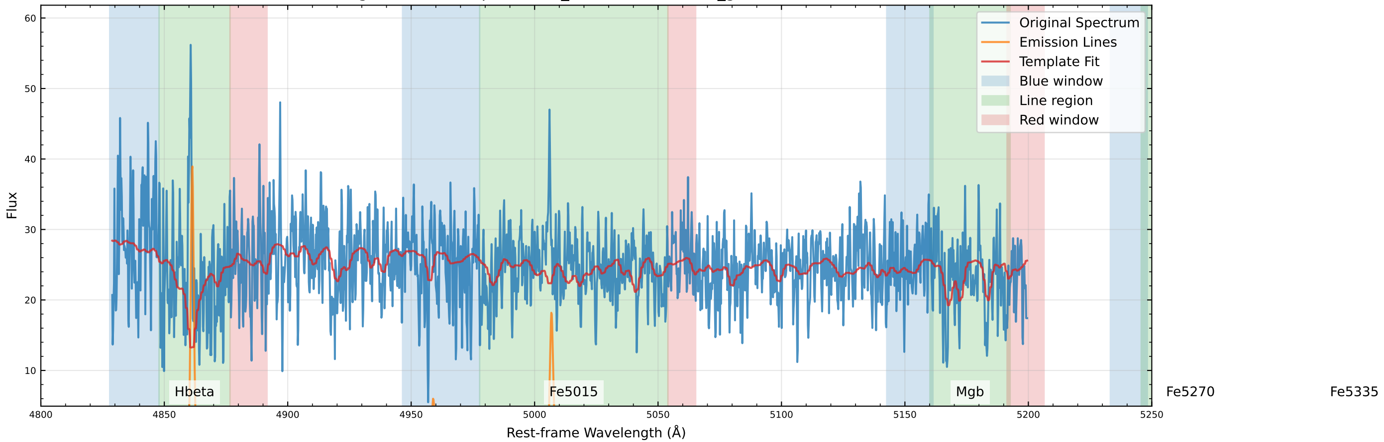
Original Data Comparison (v_star=-46.8 km/s, v_gas=-50.9 km/s)
